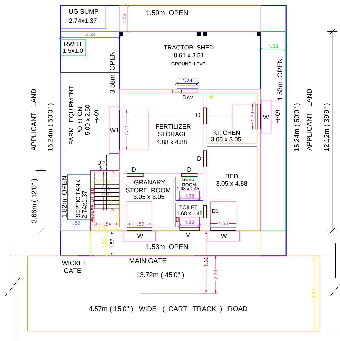
SITE CUM GROUND FLOOR PLAN
