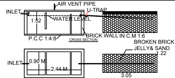
SEPTIC TANK (NOT TO SCALE)
