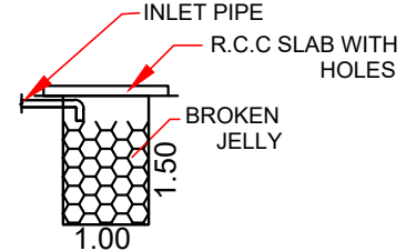
RAIN WATER HARVESTING FILTER BED
