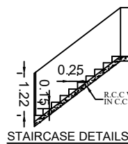
STAIRCASE DETAILS
