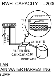
PLAN RAIN WATER HARVESTING SUMP
