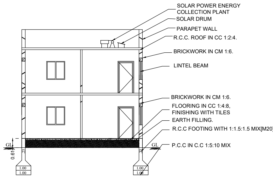
SECTION ON AB & CD
