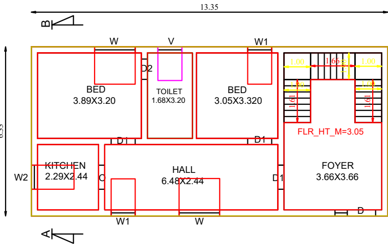
GROUND FLOOR PLAN SCALE 1 CM =1 M
