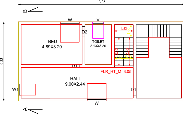
FIRST FLOOR PLAN SCALE 1 CM =1 M
