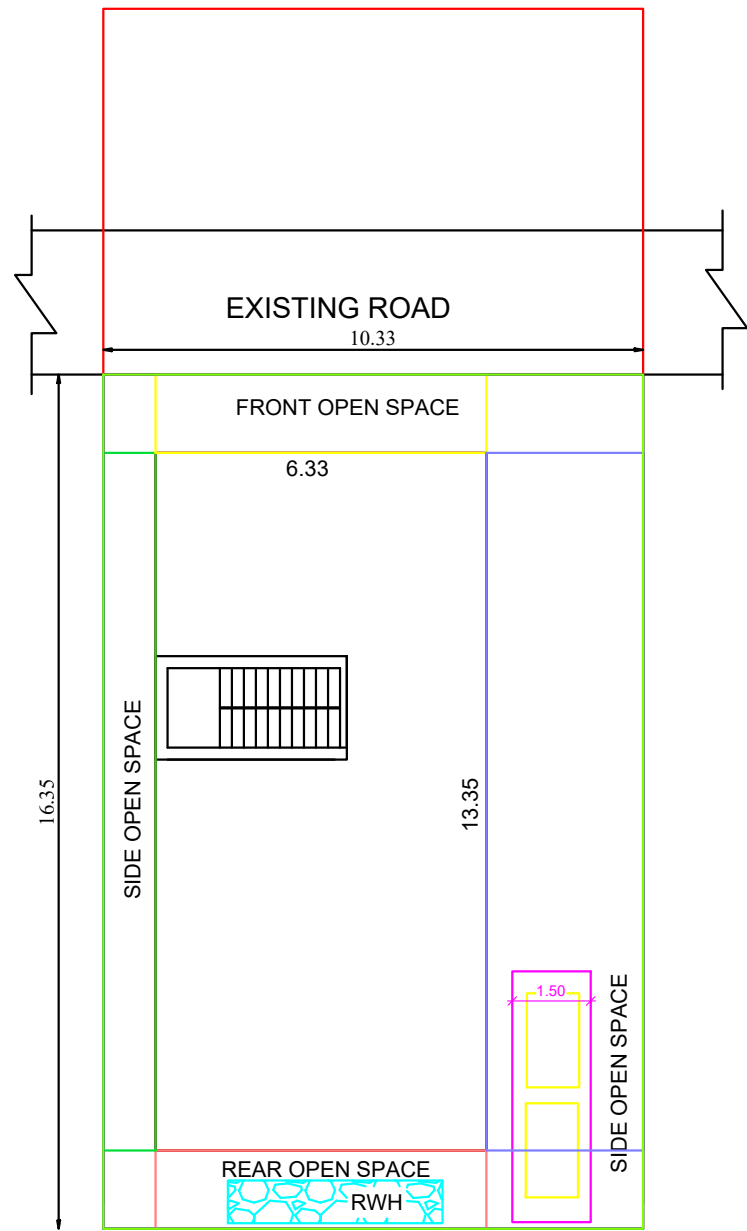
SITE PLAN SCALE 1CM:1M
