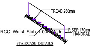
STAIRCASE DETAILS
