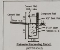
Rainwater Harvesting Trench
