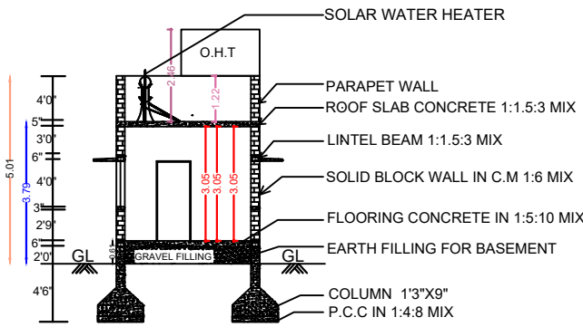
SECTION AB
