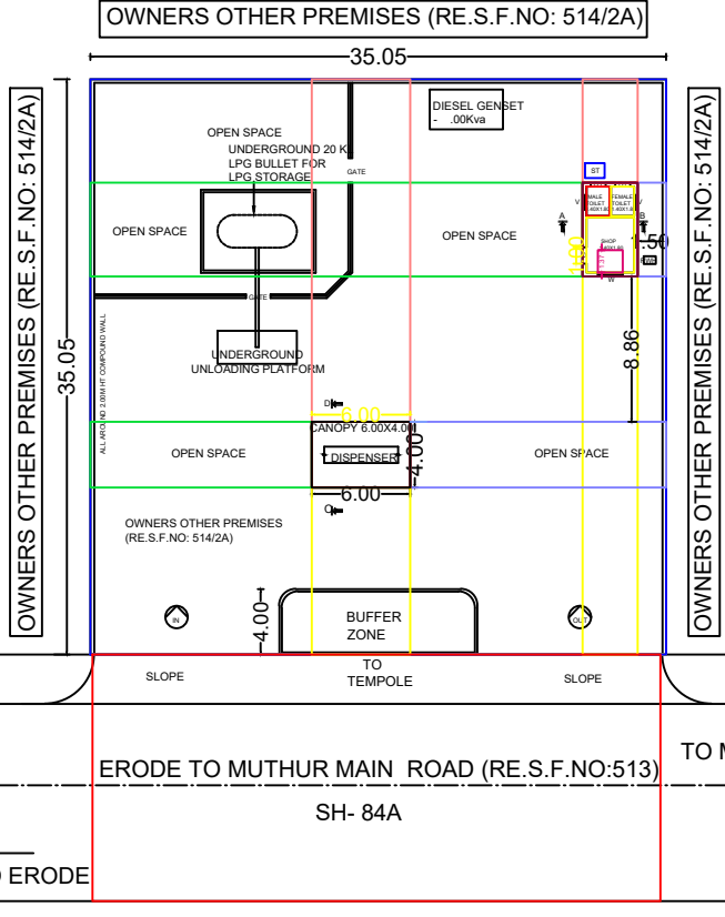
SITE CUM GROUND FLOOR PLAN(SCALE 1:100)
