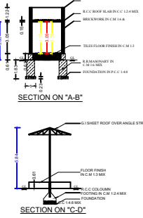
SECTION ON "C-D"
