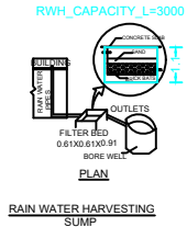
RAIN WATER HARVESTING SUMP
