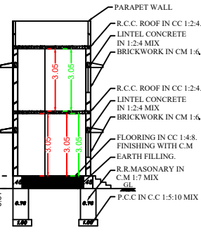
SECTION HK'
