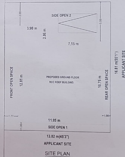
SITE PLAN
