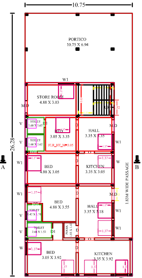
GROUND FLOOR PLAN FLR_HUT=0.05
