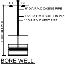
BORE WELL
