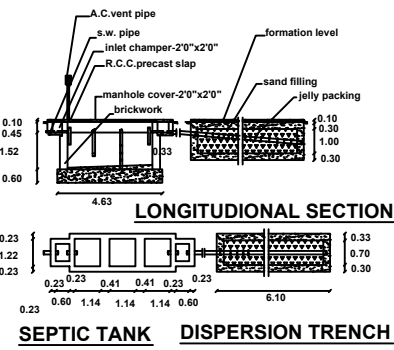
SEPTIC TANK DISPERSION TRENCH PLAN
