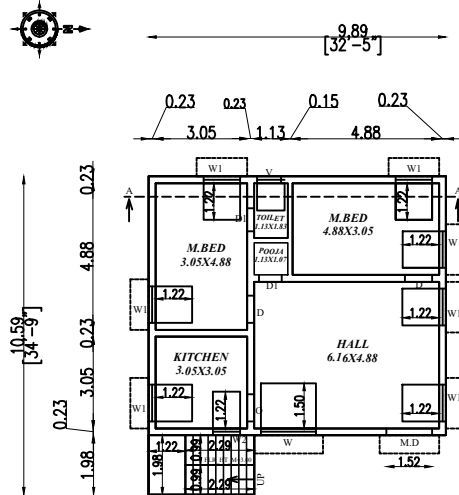
GROUND FLOOR PLAN (SCALE 1:100)
