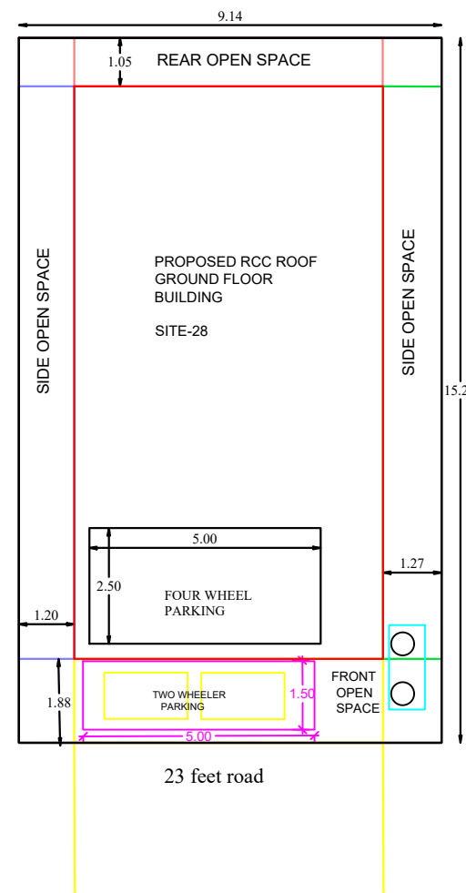
SITE & LOCATION PLAN SCALE - 1: 100
