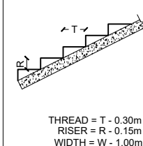
STAIRCASE DETAILS
