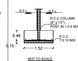
COLUMN POST DETAILS
