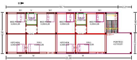
FLR_HT_m=3.05 GROUND FLOOR PLAN SCALE 1:100
