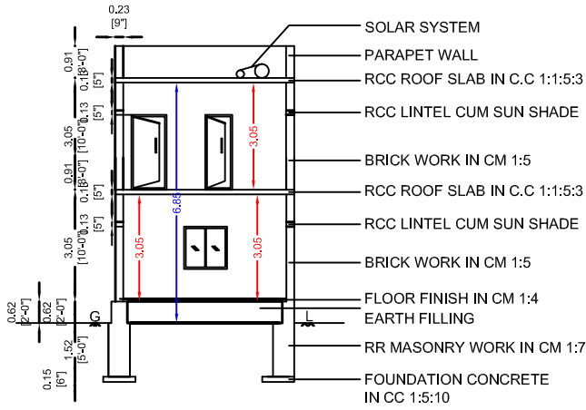
SECTION "AA" & "BB"
