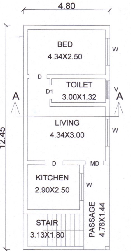
PLAN OF GROUND FLOOR
