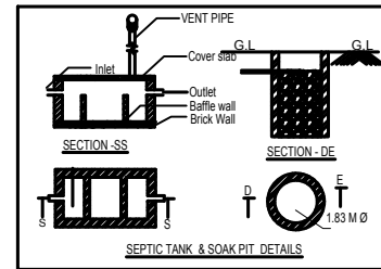
SEPTIC TANK & SOAK PIT DETAILS
