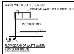
WASTE WATER COLLECTION, OHT, DRINKING WATER COLLECTION, OHT, R.C.C BUILDING, O.P., T.W.C.S. RCT, FLOW DIAGRAM OF WASTE WATER RECYCLING & REUSE
