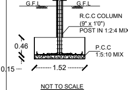
COLUMN POST DETAILS
