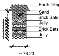
SECTION ON B-B.
