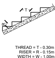
STAIRCASE DETAILS
