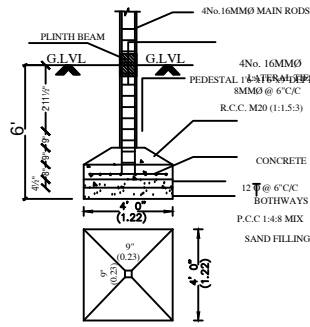
FOUNDATION DETAIL
