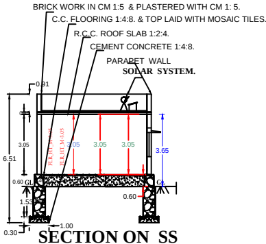
SECTION ON SS
