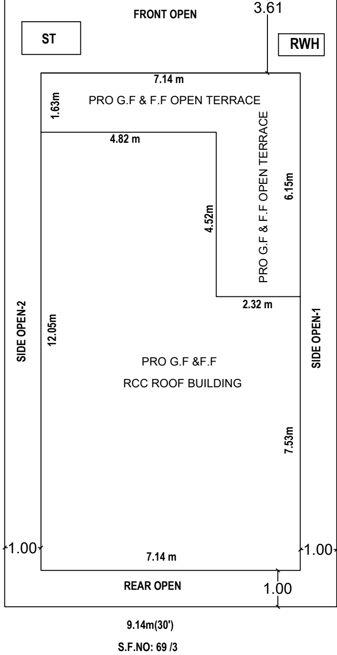
SITE PLAN
