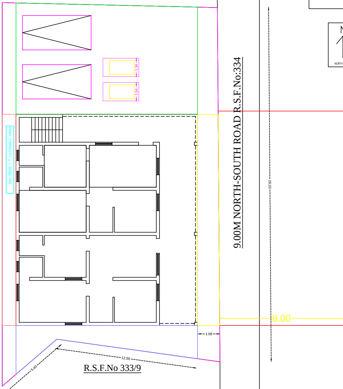
SITE CUM GROUND FLOOR PLAN
