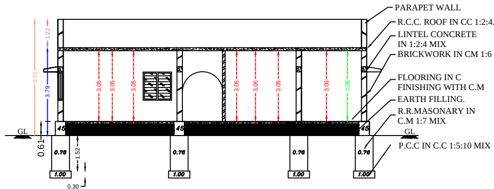
SECTION AB
