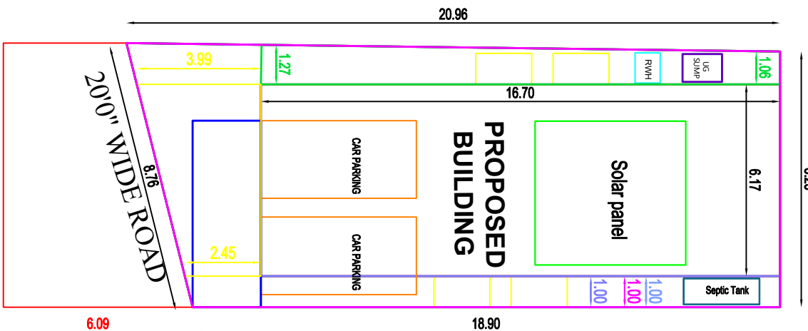
SITE PLAN
