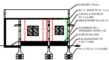
SECTION HK'
