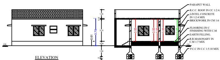
SECTION HK'
