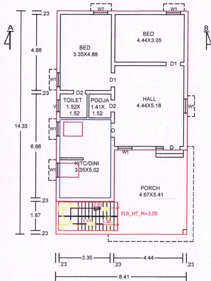
GROUND FLOOR PLAN SCALE 1 CM = 1 M
