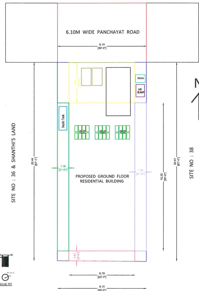
SITE PLAN 1: 100
