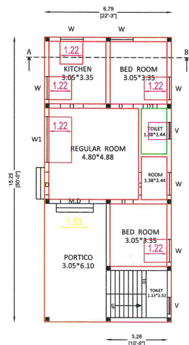
PROPOSED GROUND FLOOR BUILDING PLAN 1: 100
