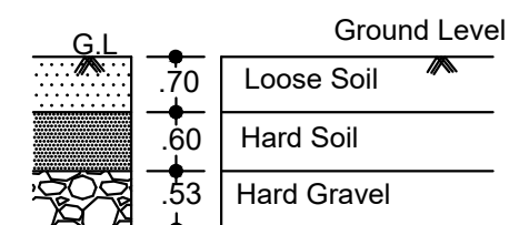
TRIAL PIT DETAILS (NOT TO SCALE)
