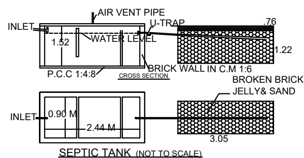
SEPTIC TANK (NOT TO SCALE)
