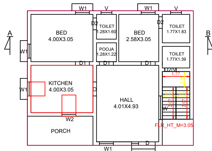
GROUND FLOOR PLAN SCALE 1 CM = 1 M
