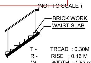
STAIR DETAILS :-
