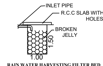
RAIN WATER HARVESTING FILTER BED
