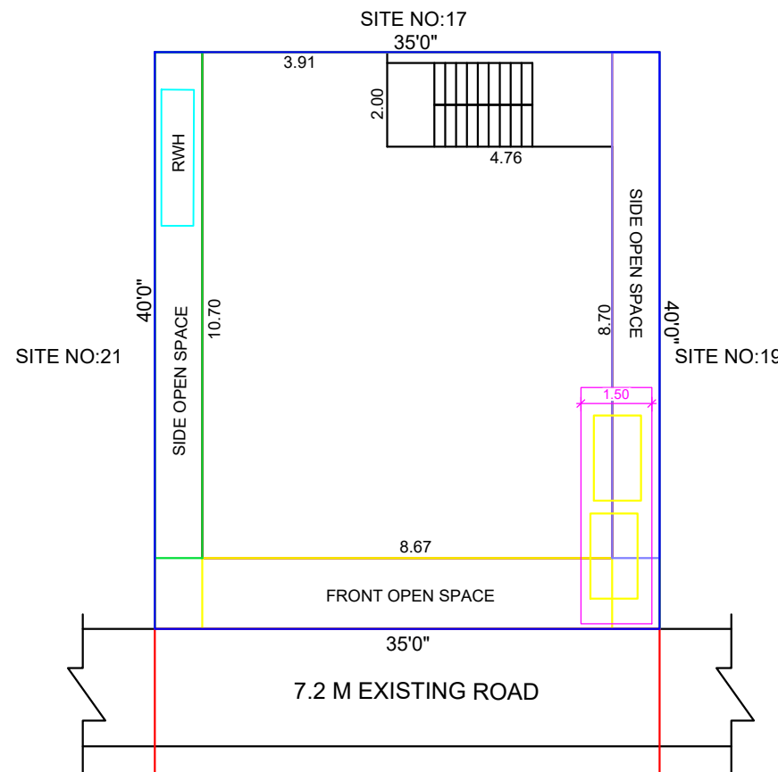
SITE PLAN SCALE 1CM:1M
