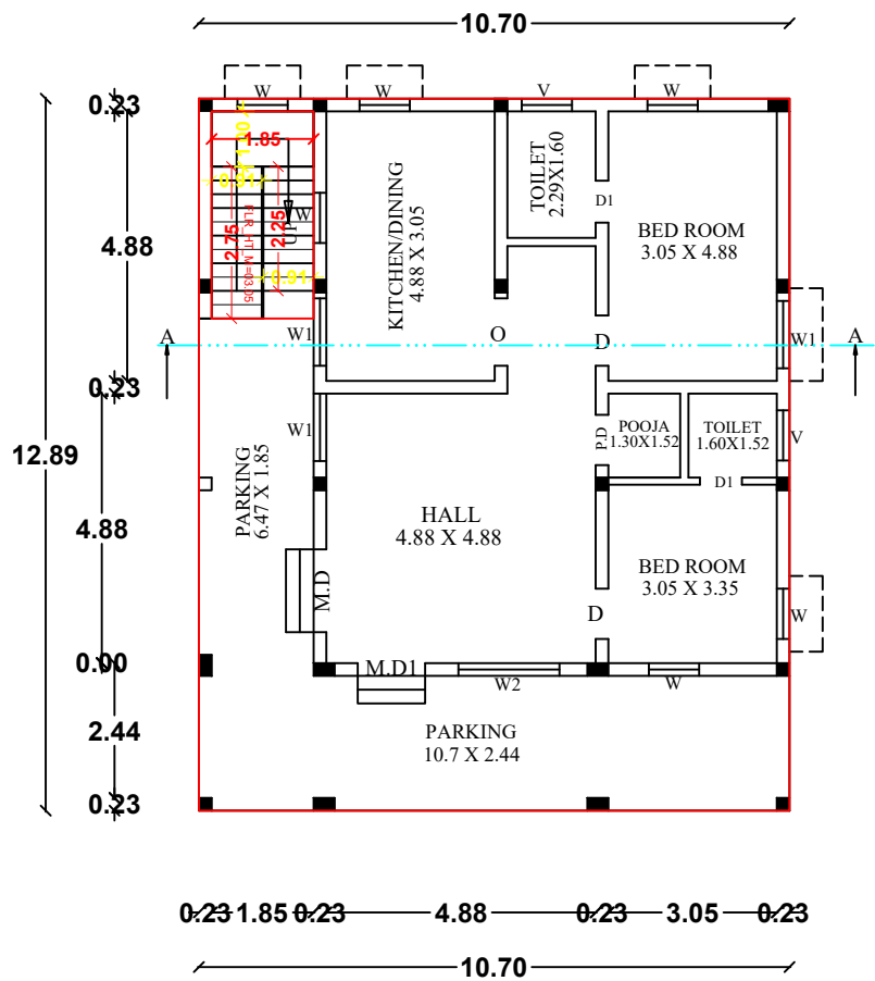
GROUND FLOOR PLAN (Existing Building)
