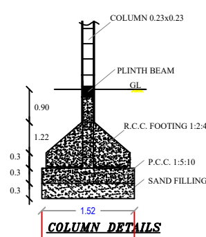
COLUMN DETAILS
