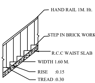
STAIR DETAIL
