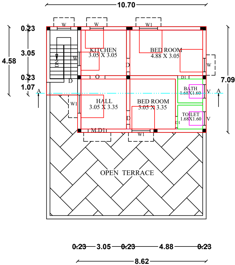
FIRST FLOOR PLAN (Proposed Building)
