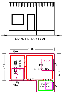
GROUND FLOOR PLAN (AC SHEET ROOF) SCALE 1:100
