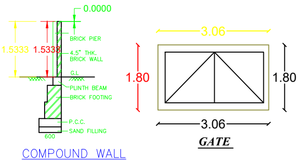
GATE
