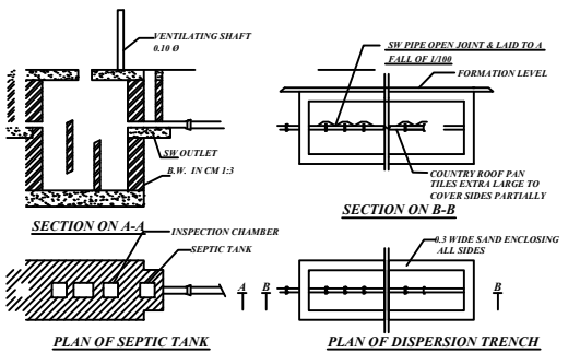
DETAILED DRAWING FOR A SEPTIC TANK WITH DISPERSION TRENCH 225 GALLONS CAPACITY OF 1000 LITRES
