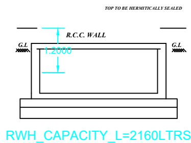
COMPOUND WALL
