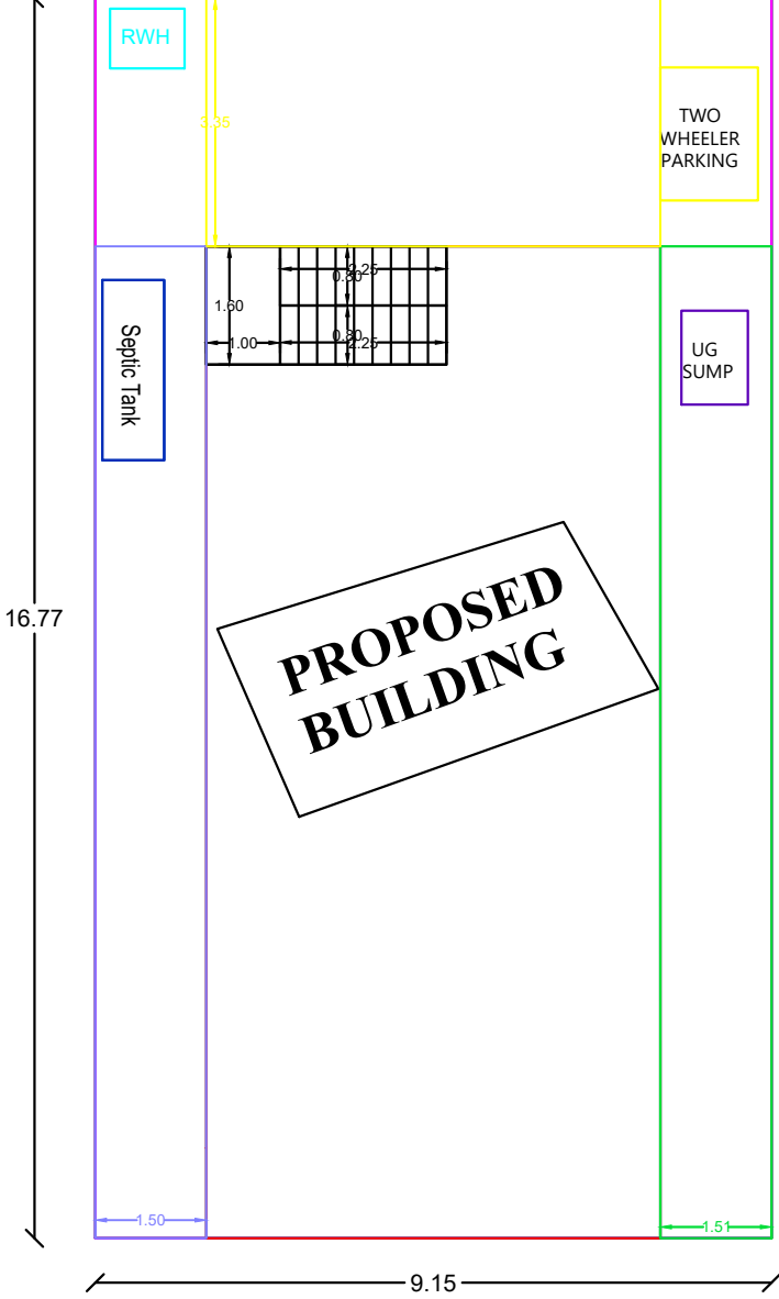
SITE PLAN
