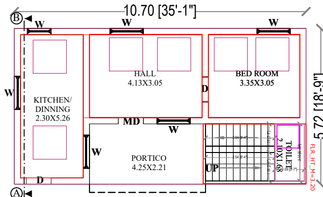
GROUND FLOOR RCC PLAN
