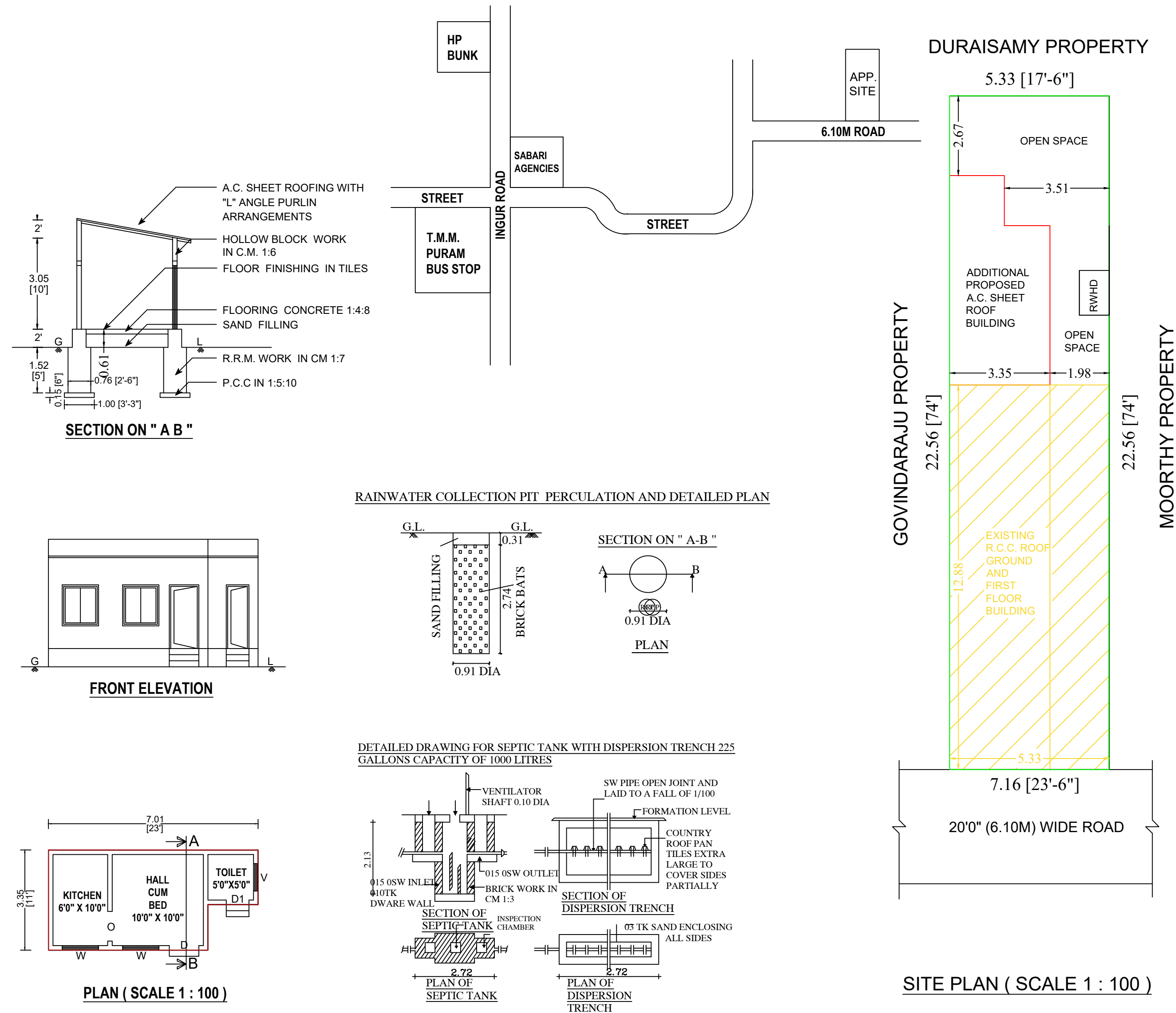
KEY PLAN
