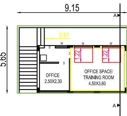
FIRST FLOOR PLAN (Scale 1:100)
