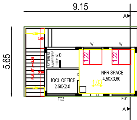
GROUND FLOOR PLAN (Scale 1:100)
