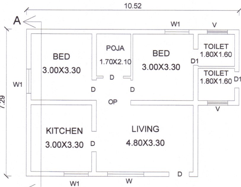
PLAN OF GROUND FLOOR
