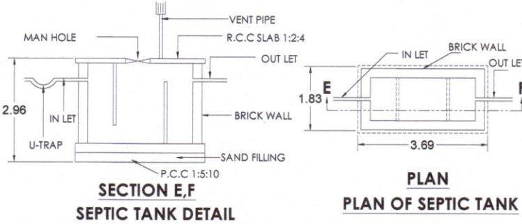
SECTION E.F SEPTIC TANK DETAIL
