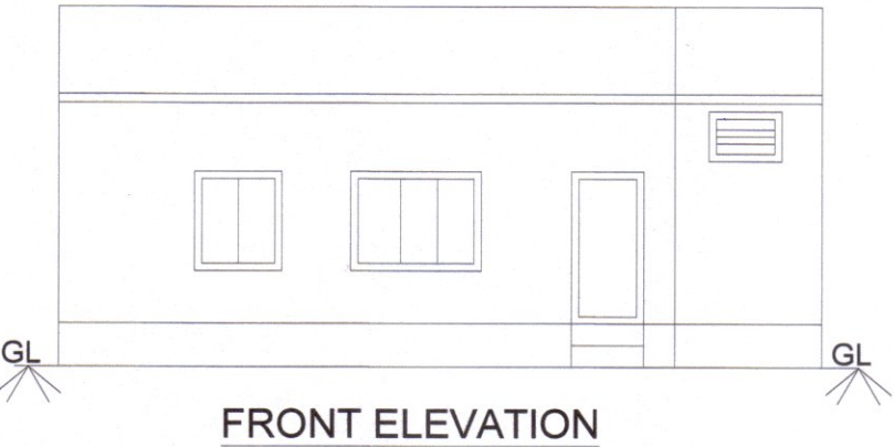
FRONT ELEVATION
