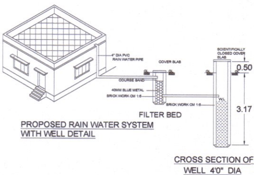
CROSS SECTION OF WELL 40" DIA
