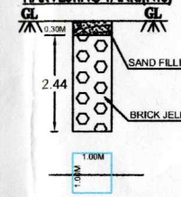
DETAILS OF RAINWATER HARVESTING TANK (NTS)
