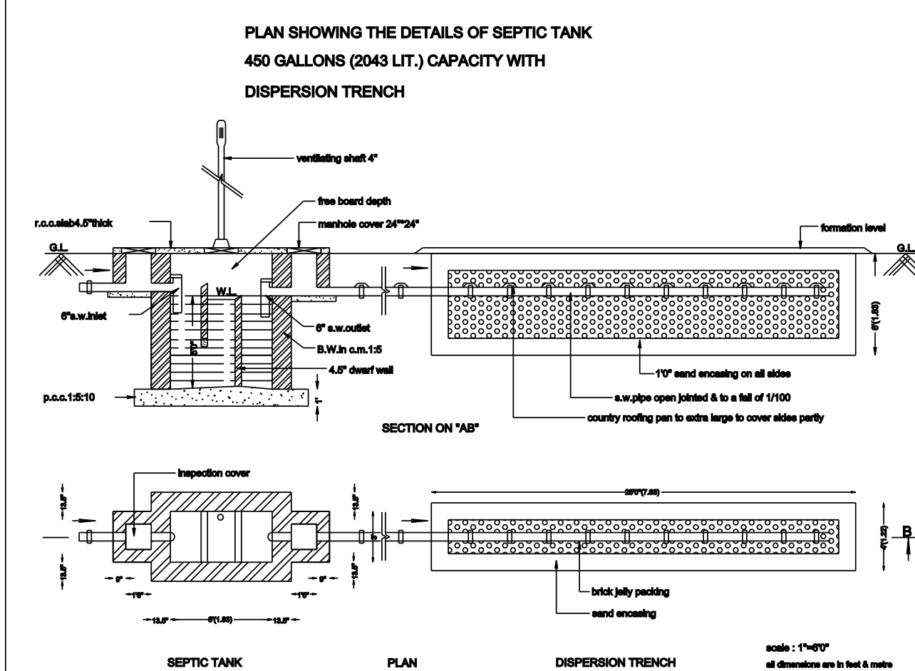
SECTION VIEW
