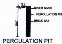
PERCOLATION PIT
