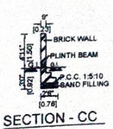
SECTION - CC
