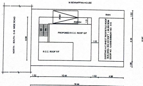
SITE PLAN
