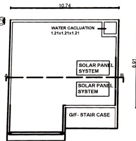
TERRACE ROOF PLAN
