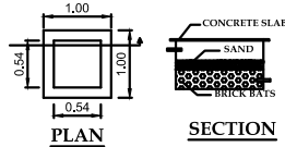
RAIN WATER HARVESTING TANK
