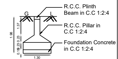
PILLAR DETAILS (Not to Scale)
