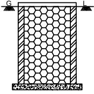
SEPTIC TANK - 3.05 x 1.07m (Scale-1cm=1m)
