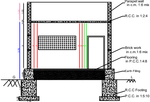
SECTION BB1
