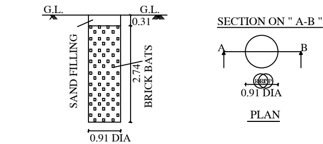
RAINWATER COLLECTION PIT PERCUSSION AND DETAILED PLAN
