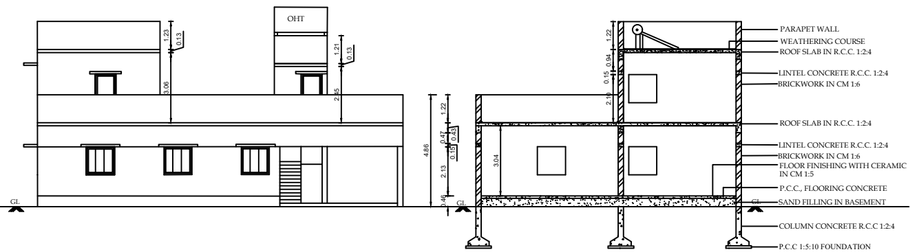
FRONT ELEVATION
