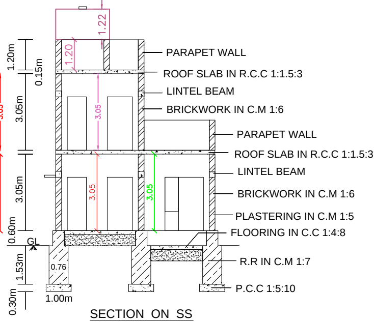
SECTION ON SS
