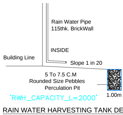
RAIN WATER HARVESTING TANK DETAILS
