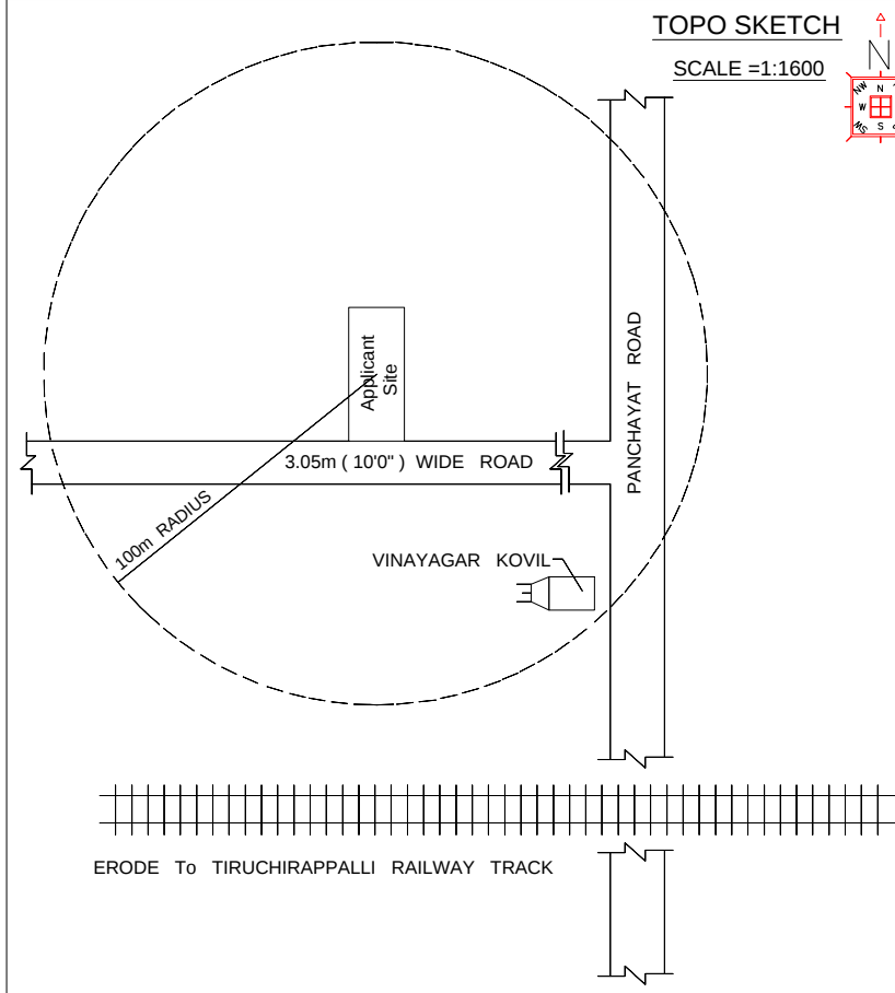
TOPO SKETCH SCALE = 1:1600
