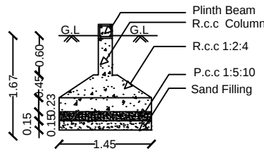
COLUMN FOOTING DETAILS
