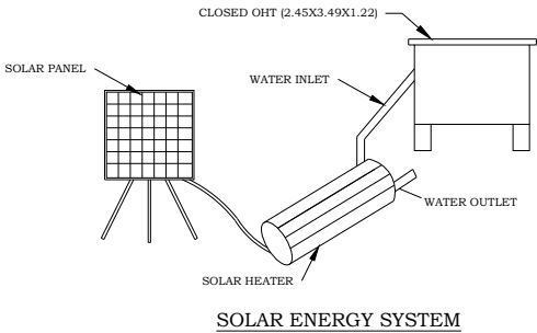
SOLAR ENERGY SYSTEM
