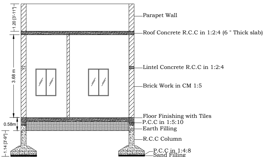
SECTION X-X
