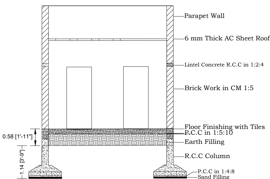
SECTION X-X
