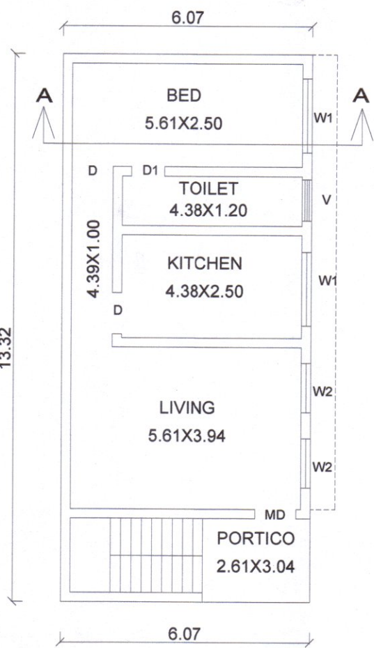
PLAN OF GROUND FLOOR
