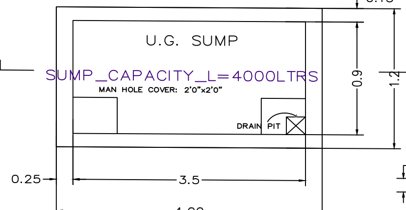
PLAN OF SUMP DETAIL
