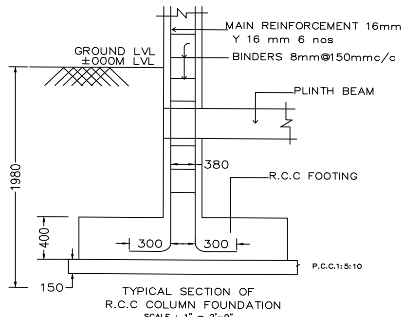
TYPICAL SECTION OF R.C.C. COLUMN FOUNDATION
